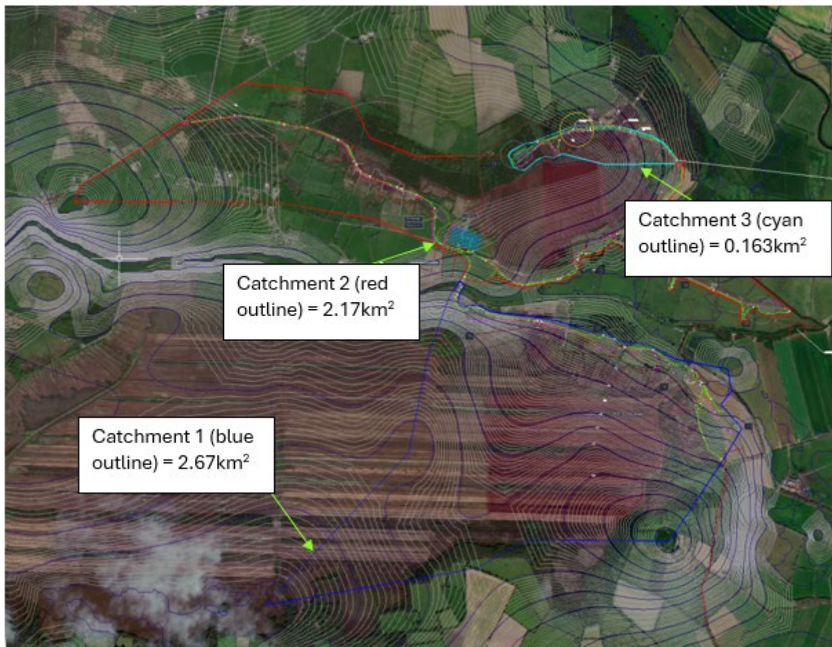
Figure 12-12: Run-off catchment areas
