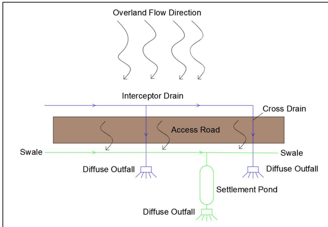
Figure 12-11: Drainage Design Principles
